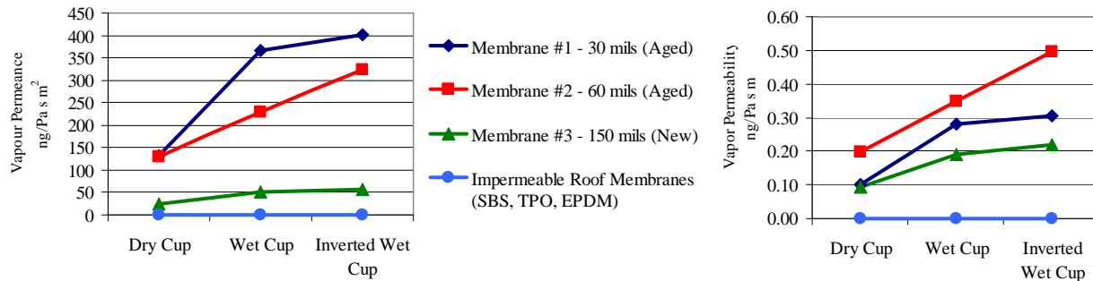
Figure 10: ASTM E96 - Vapour Permeability and Permeance Laboratory Results for Membrane Samples
