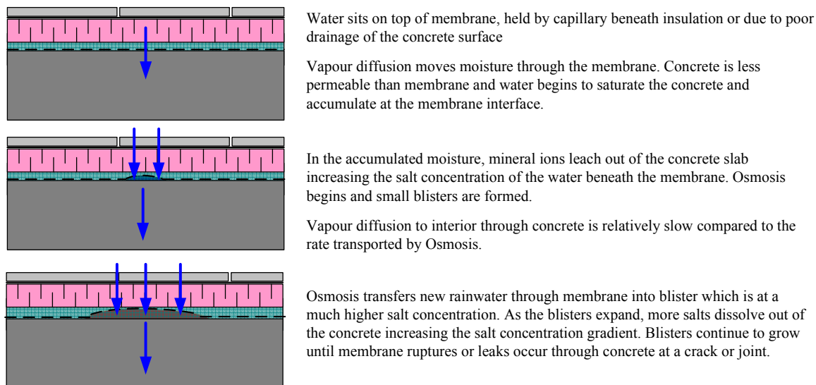
Figure 9: Blister Formation Mechanism by Osmosis
