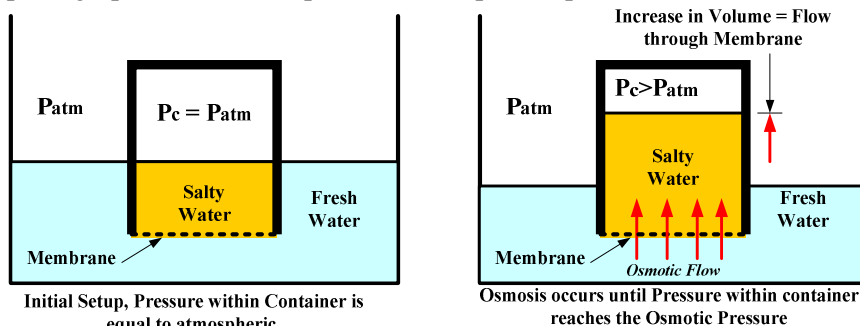
Figure 13: Osmotic Flow Testing Apparatus Schematic
