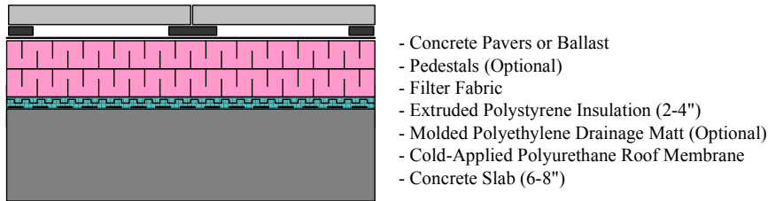
Figure 6: Typical IRMA Waterproofed with a Polyurethane Membrane
